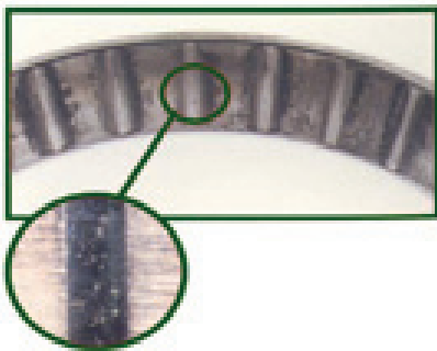
Figure 6 Localized wear spots made by rolling elements on raceway due to limited rolling/ repeated impact are called false brinelling.
