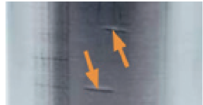
Figure 11 Raceways and rolling elements can incur indentations and nicks caused by hard, possibly sharp, objects.
