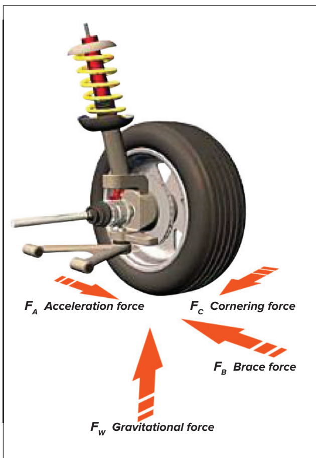
Picture 1 Wheel affecting forces
